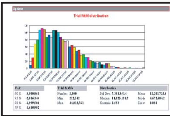
VaR Statistics
